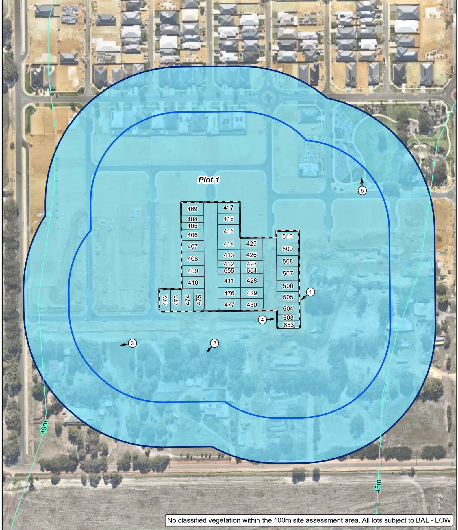
Figure 1: Vegetation Classification
